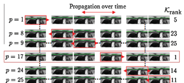
Fig. 2. Slice segmentation in SCR algorithm: for each frame p = 1, \dots, P , recover a contour using Dijkstra's algorithm in polar space, propagate the contour to all other frames, and repeat. Choose the combination of contours (in this case recovered from frame 17) with the lowest cost.
