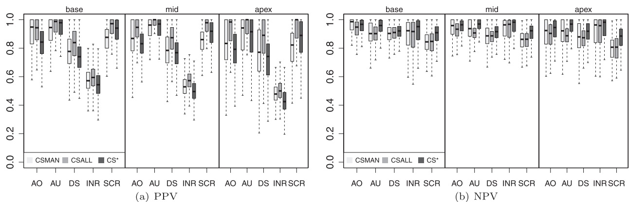
Fig. 6. Comparison of PPV and NPV values from each rater between CSMAN and CSALL consensus.
