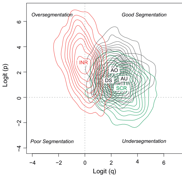
Fig. 9. Distributions of sensitivity and specificity values after Logit transformation (13). The value of Logit (0) is equal to sensitivity/specificity at 0.5. Therefore regions centered at the origin (dashed lines) define four characteristics of segmentation results. The rater labels are at the peak of each distribution, with the colors are: INR in red, SCR in green, and manual raters (AU, AO and DS) in black. (For interpretation of the references to colour in this figure legend, the reader is referred to the web version of this article.)
